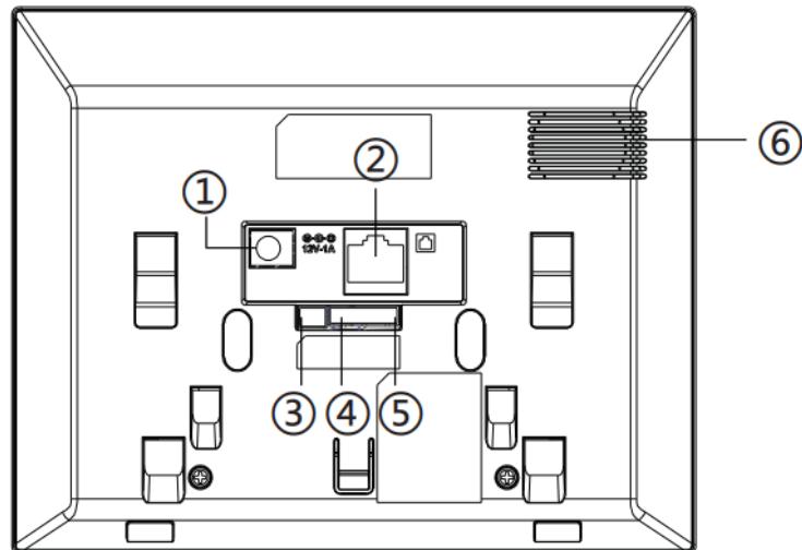
Picture 2 - interface
