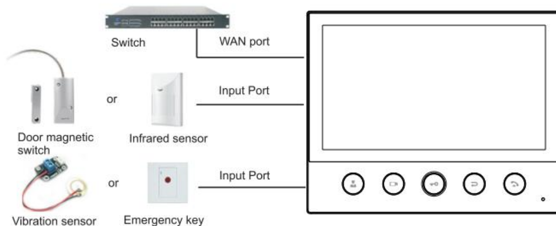
Picture 1 - Peripheral connection diagram
